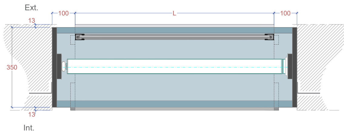
Enrollamiento Interior
