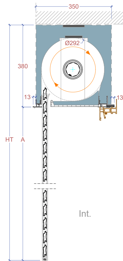
Enrollamiento Interior
