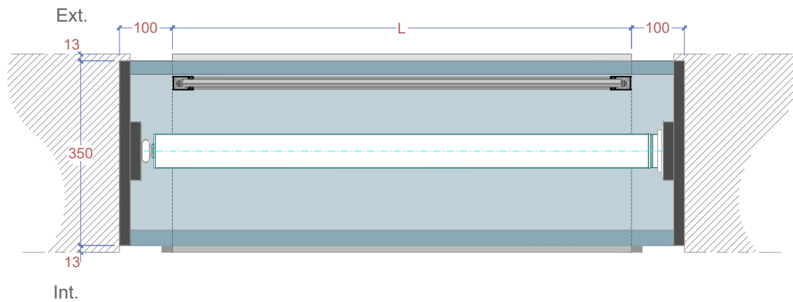
Enrollamiento Interior
